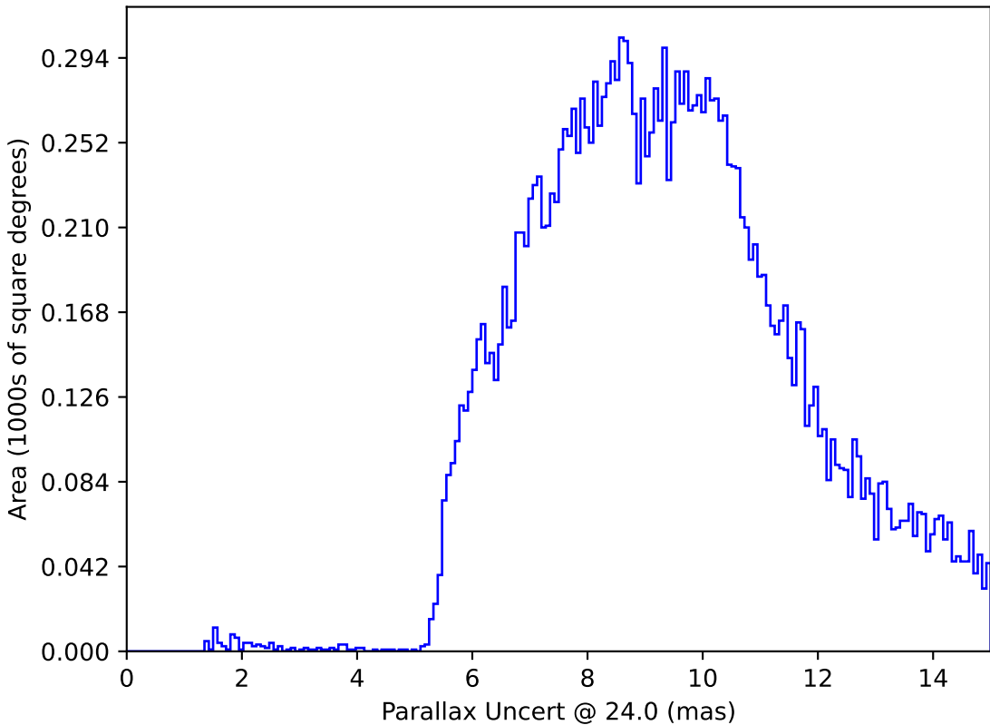
weather_cloudso31v3.4_10yrs : Parallax Uncert @ 24.0
