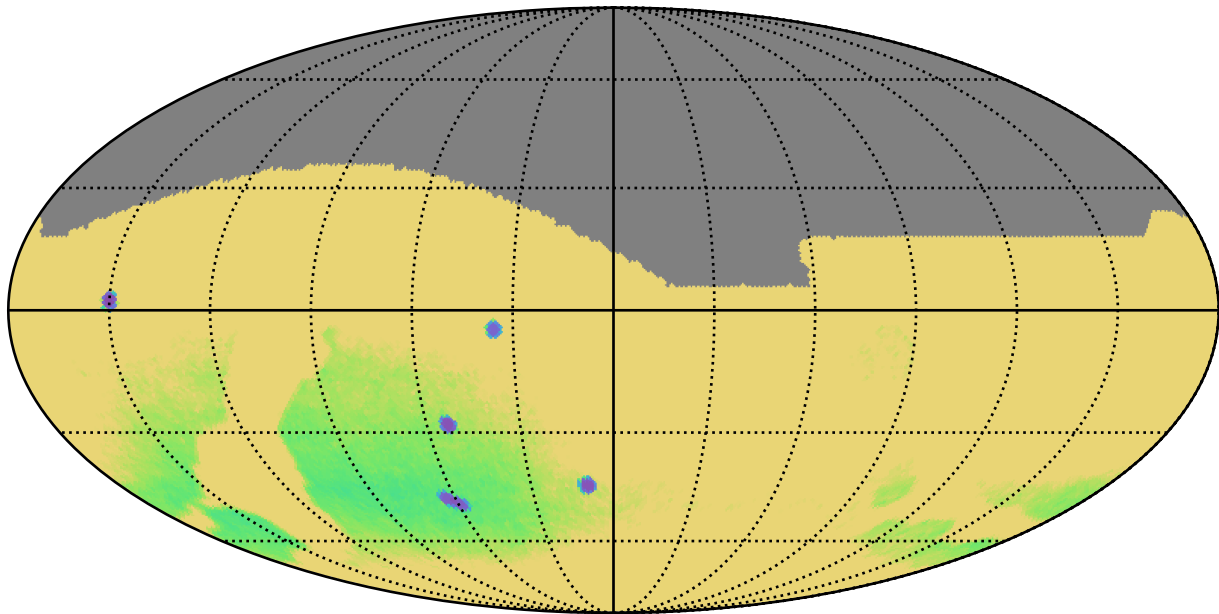
weather_cloudso31v3.4_10yrs : Parallax Uncert @ 22.4
