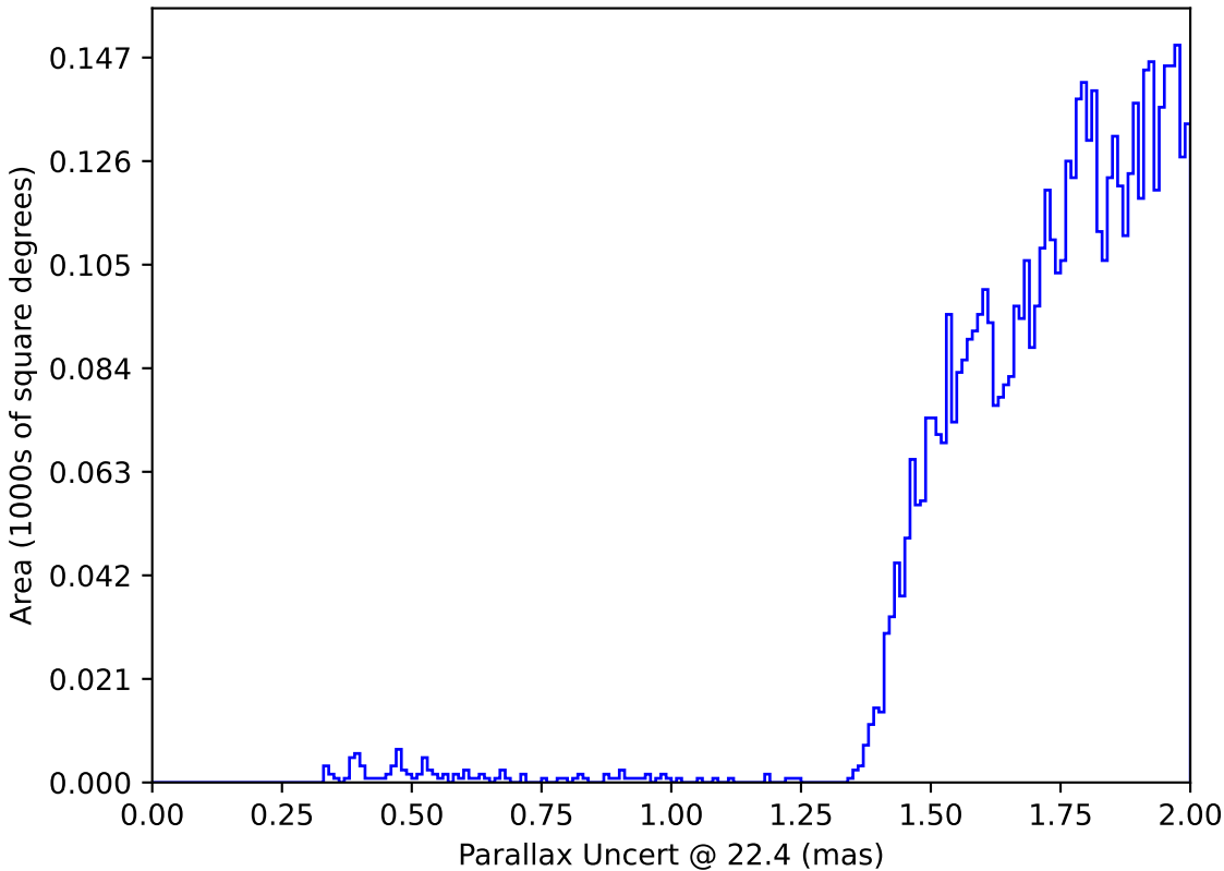
weather_cloudso31v3.4_10yrs : Parallax Uncert @ 22.4
