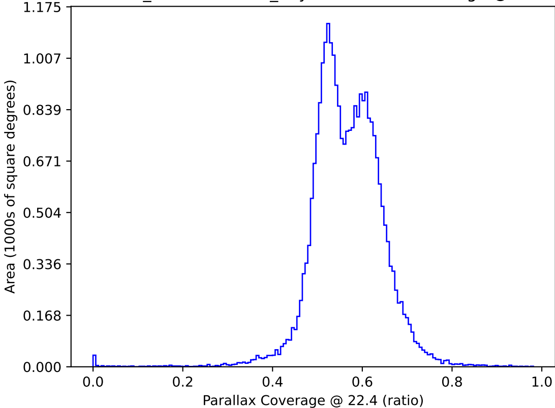
weather_cloudso31v3.4_10yrs : Parallax Coverage @ 22.4
