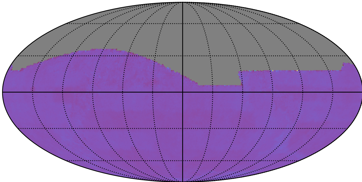
weather_cloudso31v3.4_10yrs : Normalized Proper Motion Uncert @ 24.0
