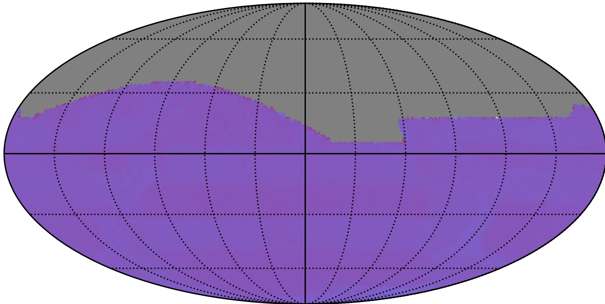
weather_cloudso31v3.4_10yrs : Normalized Proper Motion Uncert @ 20.5
