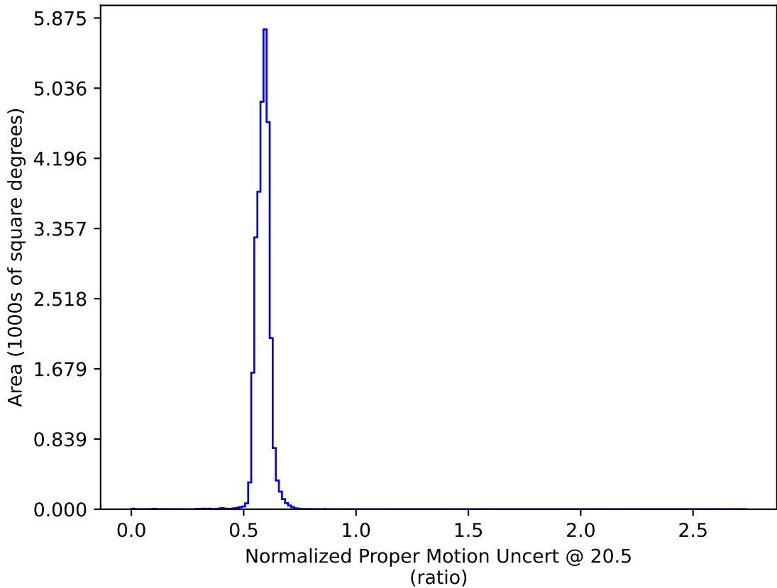
weather_cloudso31v3.4_10yrs : Normalized Proper Motion Uncert @ 20.5
