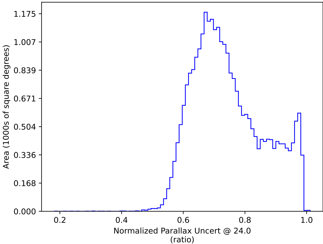
weather_cloudso31v3.4_10yrs : Normalized Parallax Uncert @ 24.0
