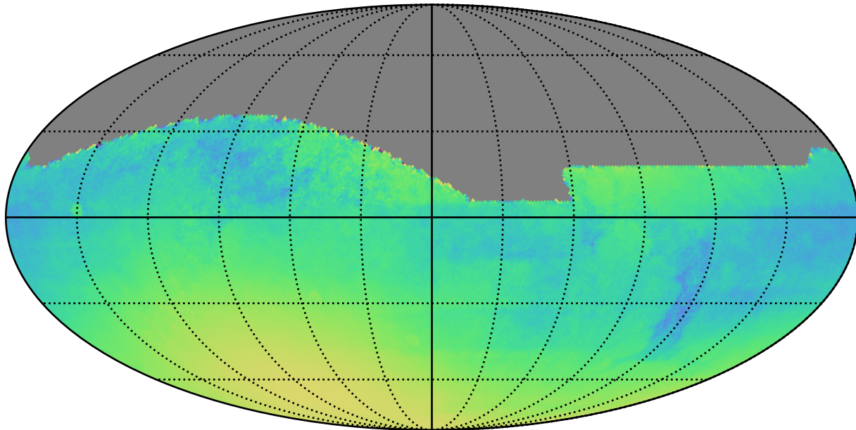
weather_cloudso31v3.4_10yrs : Normalized Parallax Uncert @ 22.4
