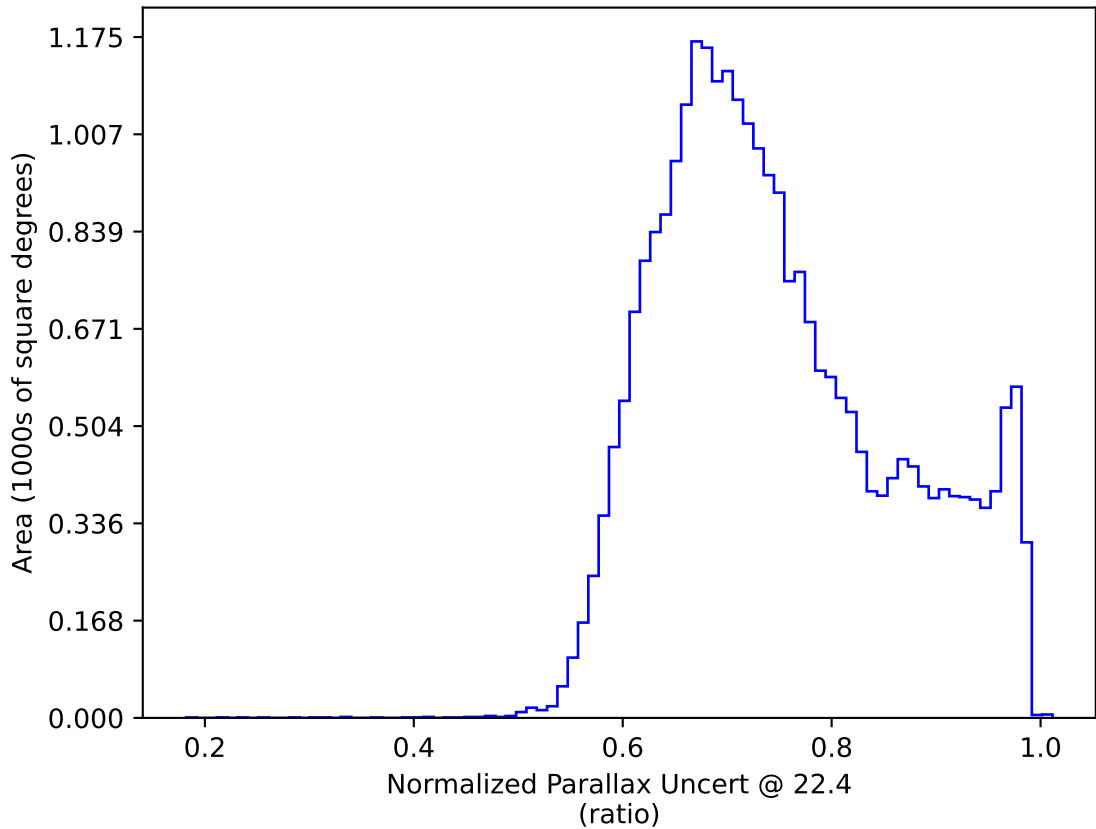
weather_cloudso31v3.4_10yrs : Normalized Parallax Uncert @ 22.4
