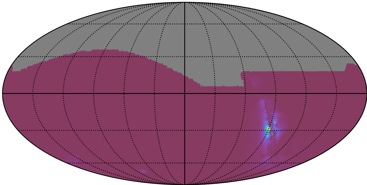
weather_cloudso31v3.4_10yrs : NlcPoints
