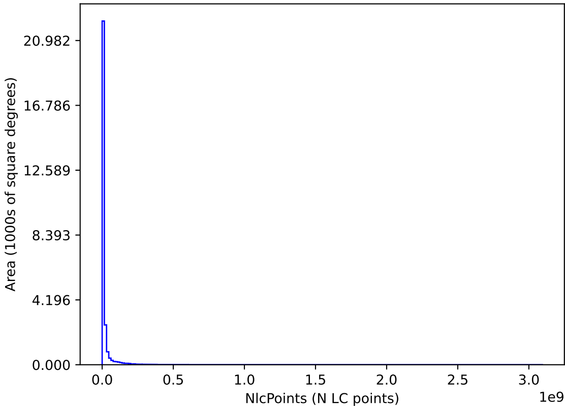
weather_cloudso31v3.4_10yrs : NlcPoints
