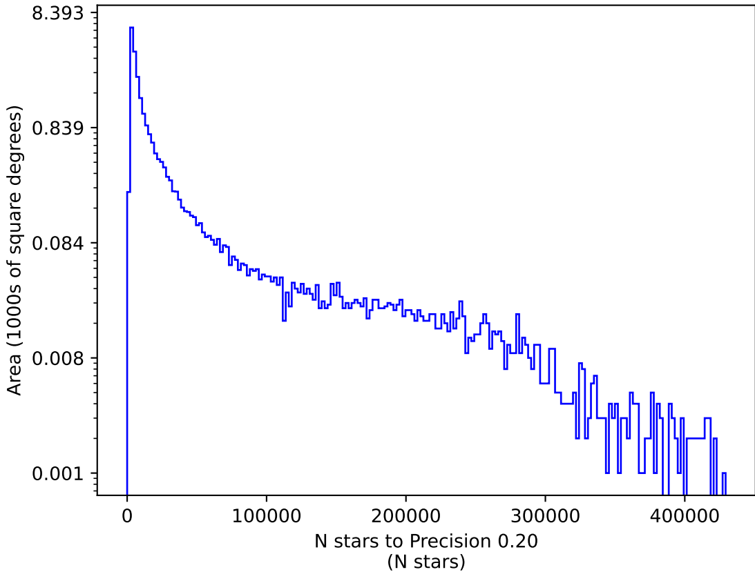
weather_cloudso31v3.4_10yrs u: N stars to Precision 0.20
