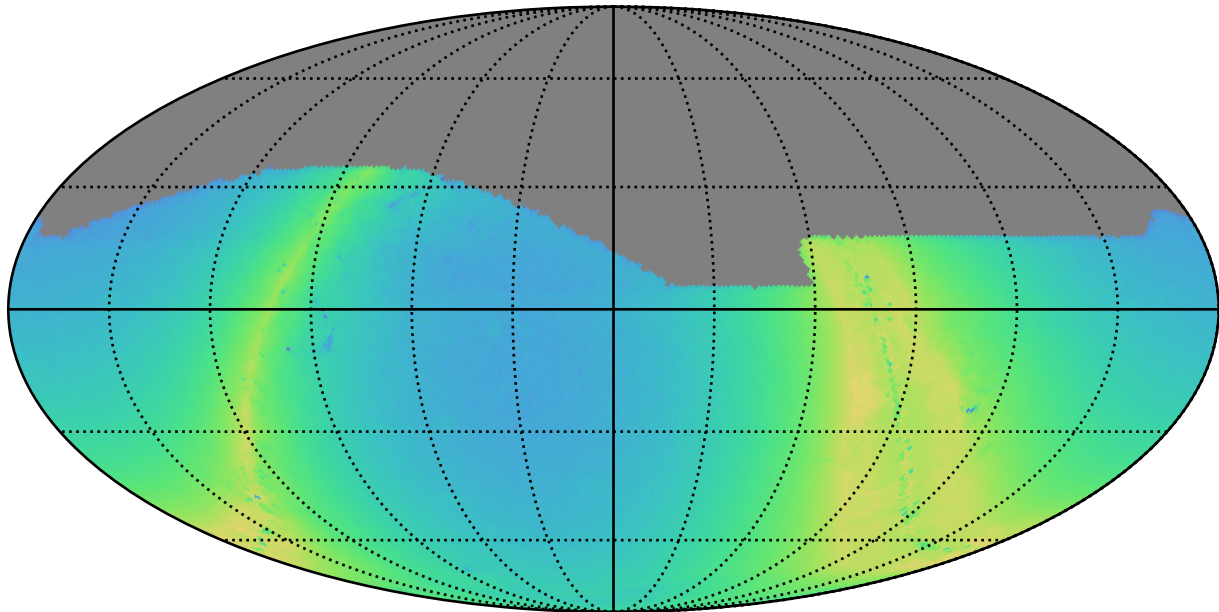
weather_cloudso31v3.4_10yrs r: N stars to Precision 0.20
