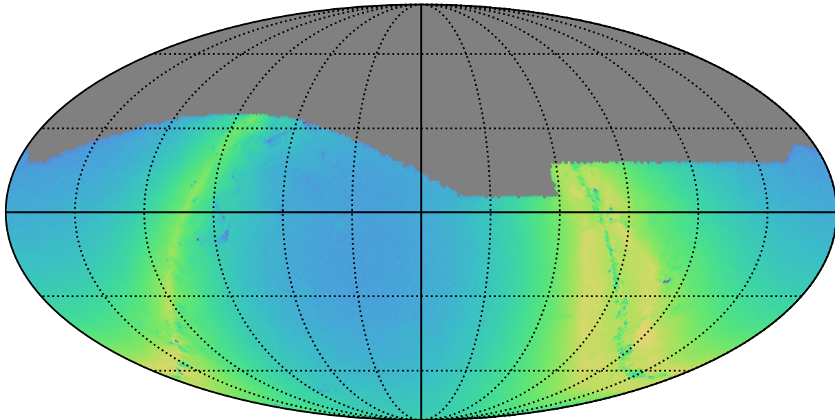
weather_cloudso31v3.4_10yrs g: N stars to Precision 0.20
