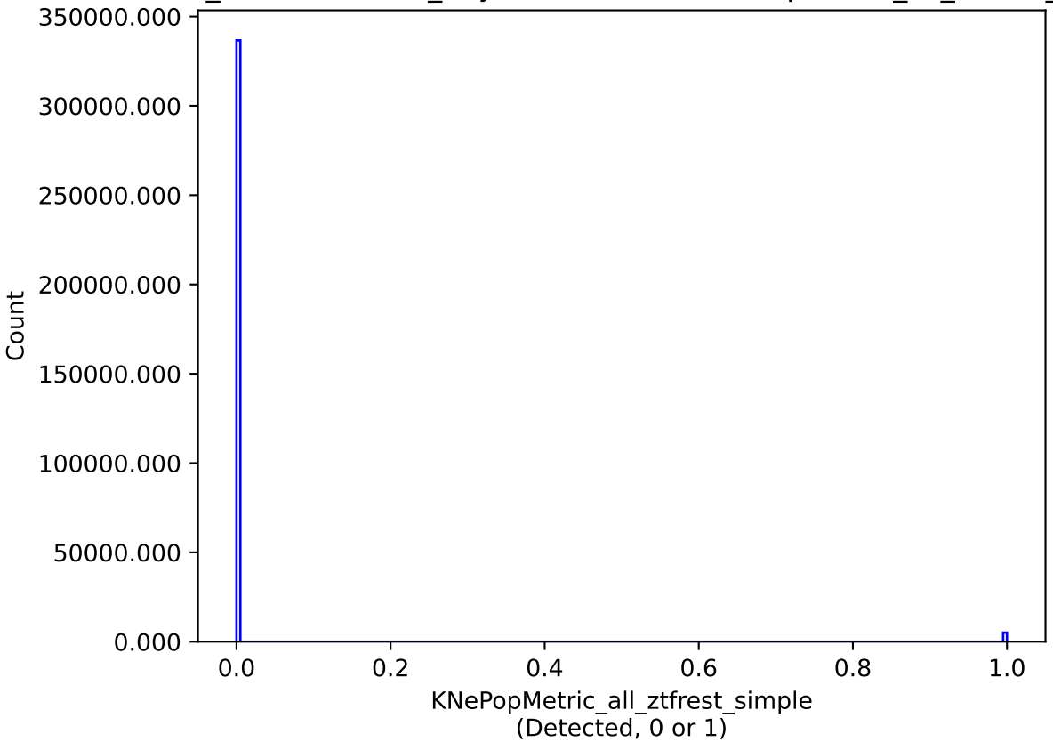
weather_cloudso31v3.4_10yrs all models: KNePopMetric_all_ztfrest_simple
