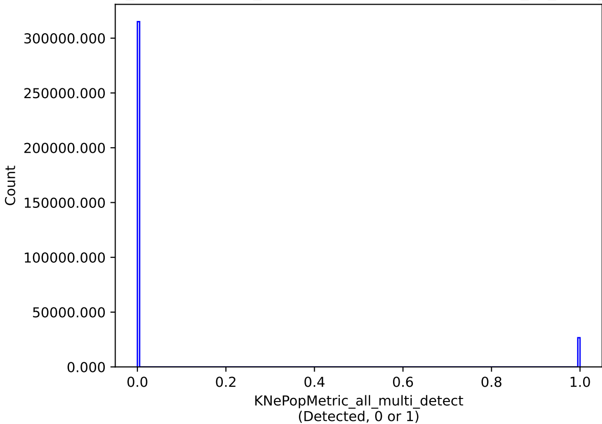
weather_cloudso31v3.4_10yrs all models: KNePopMetric_all_multi_detect
