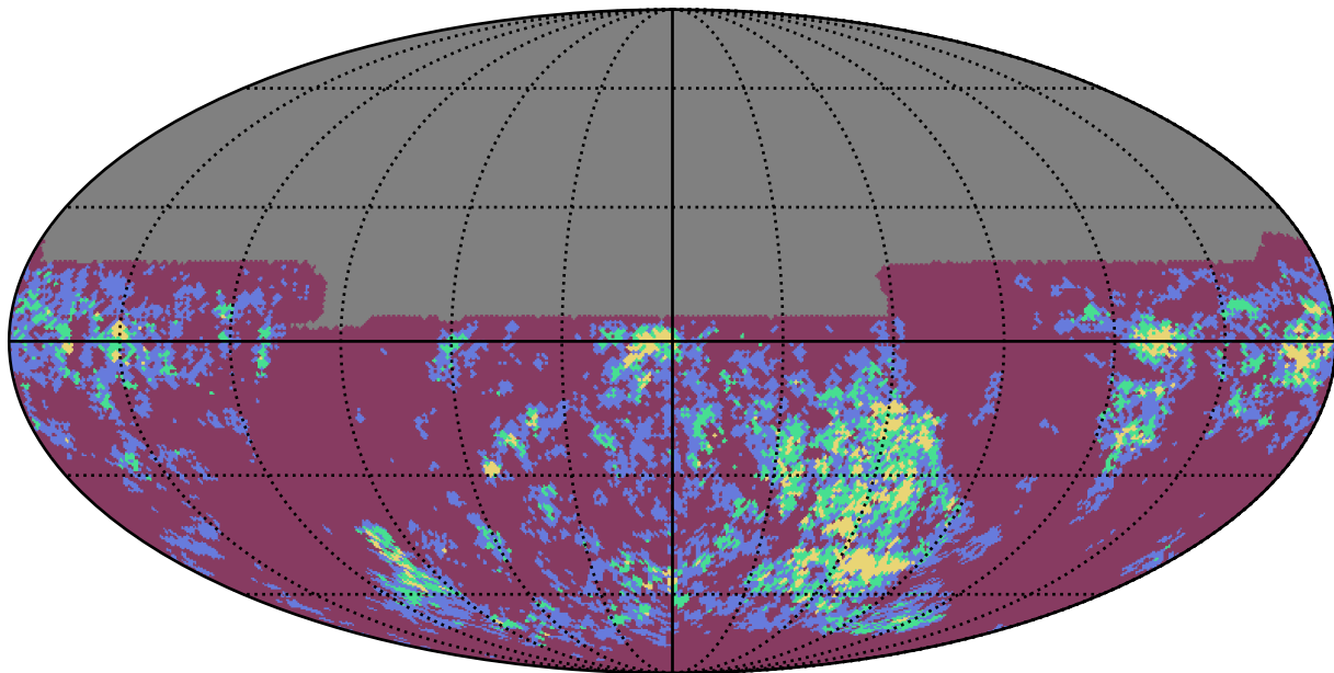
weather_cloudso31v3.4_10yrs y band: Gaps_7hr
