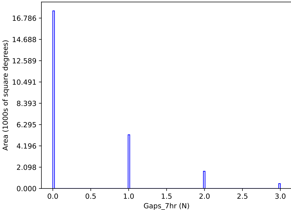
weather_cloudso31v3.4_10yrs y band: Gaps_7hr
