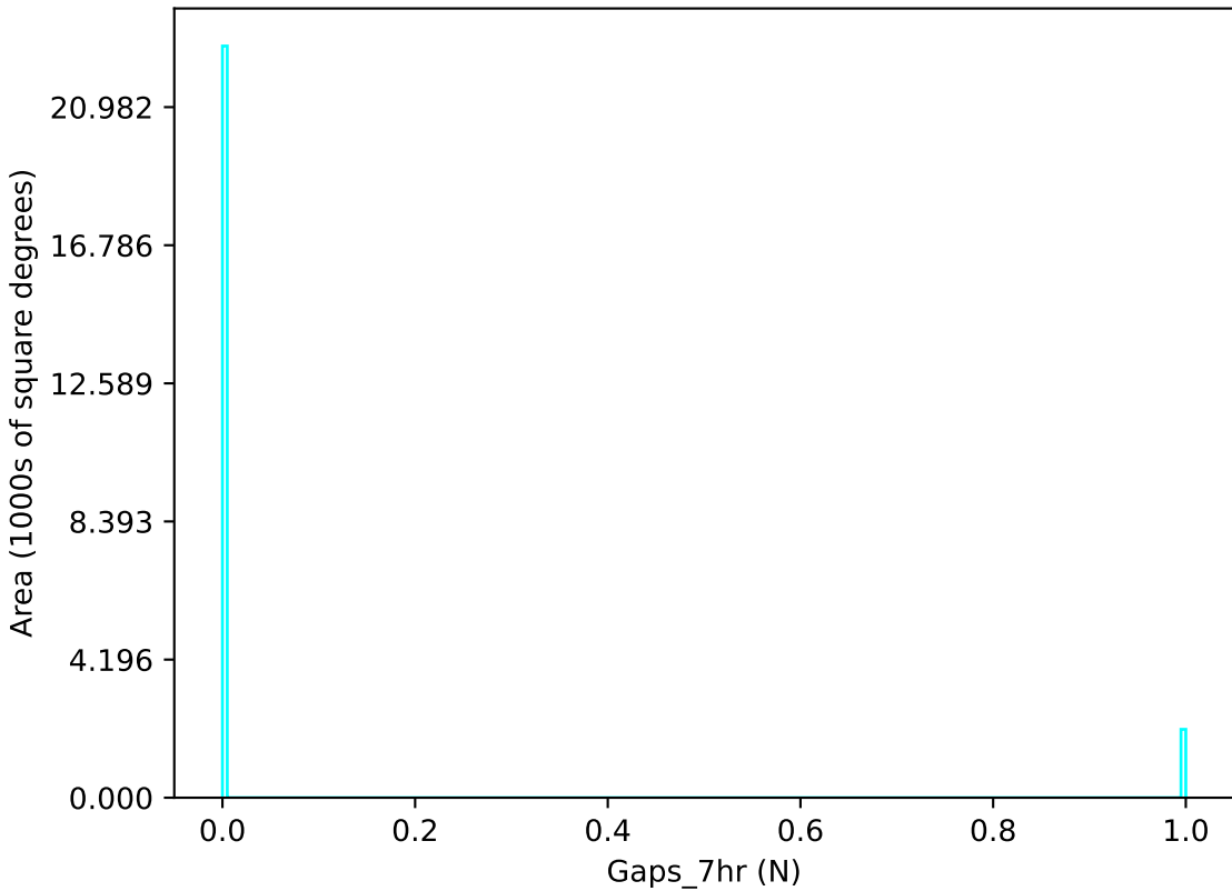
weather_cloudso31v3.4_10yrs u band: Gaps_7hr
