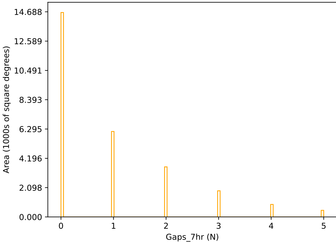
weather_cloudso31v3.4_10yrs r band: Gaps_7hr
