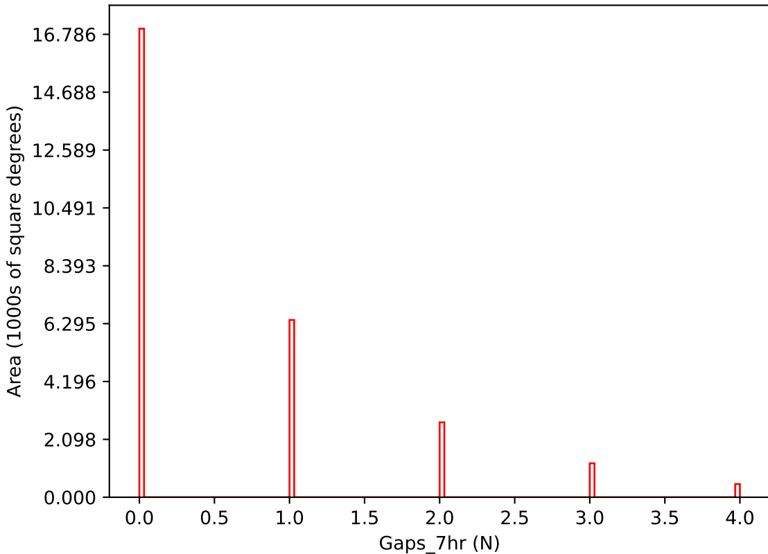
weather_cloudso31v3.4_10yrs i band: Gaps_7hr
