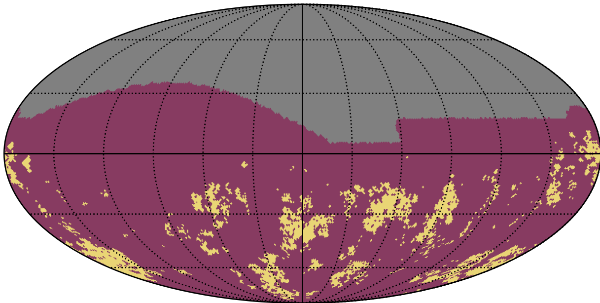
weather_cloudso31v3.4_10yrs g band: Gaps_7hr
