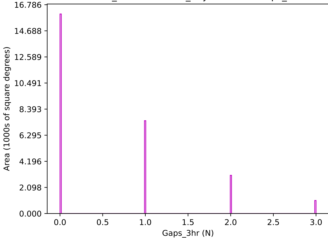
weather_cloudso31v3.4_10yrs z band: Gaps_3hr
