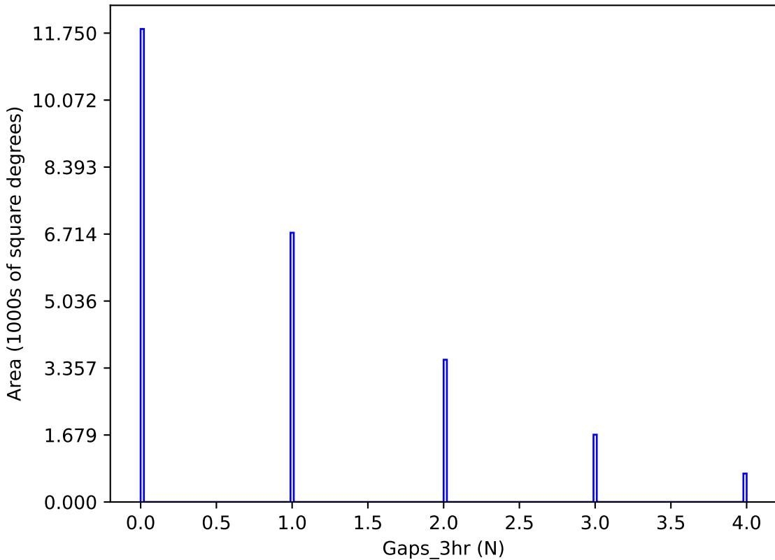
weather_cloudso31v3.4_10yrs y band: Gaps_3hr
