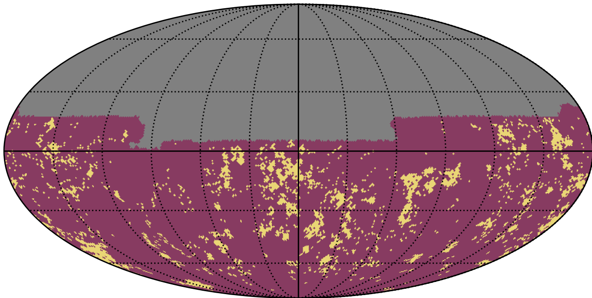
weather_cloudso31v3.4_10yrs u band: Gaps_3hr
