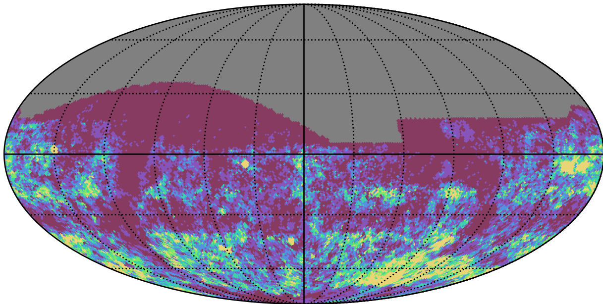
weather_cloudso31v3.4_10yrs r band: Gaps_3hr
