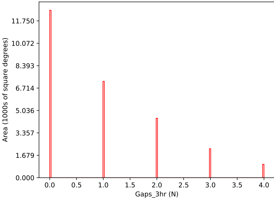
weather_cloudso31v3.4_10yrs i band: Gaps_3hr
