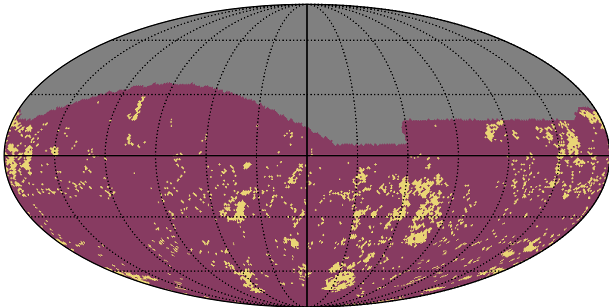
weather_cloudso31v3.4_10yrs g band: Gaps_3hr
