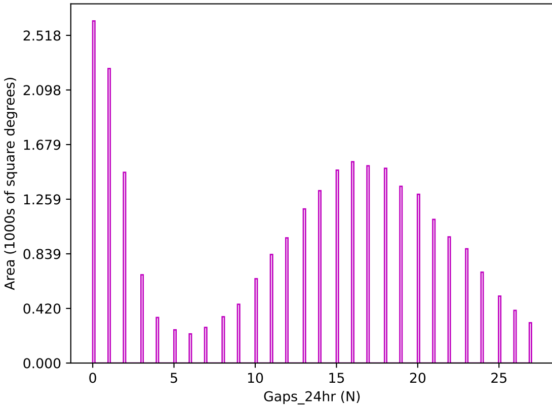
weather_cloudso31v3.4_10yrs z band: Gaps_24hr
