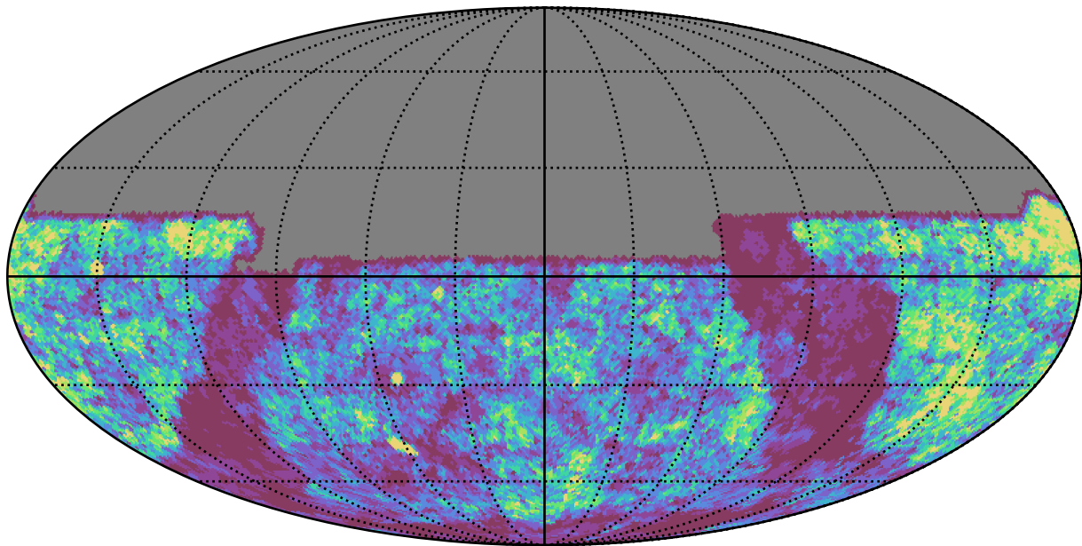
weather_cloudso31v3.4_10yrs u band: Gaps_24hr
