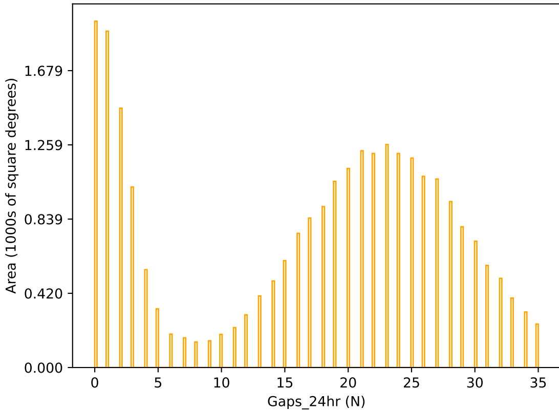
weather_cloudso31v3.4_10yrs r band: Gaps_24hr
