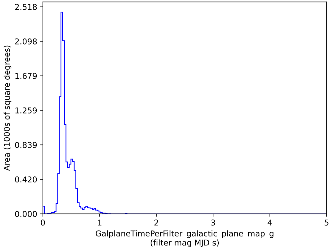
weather_cloudso31v3.4_10yrs : GalplaneTimePerFilter_galactic_plane_map_g
