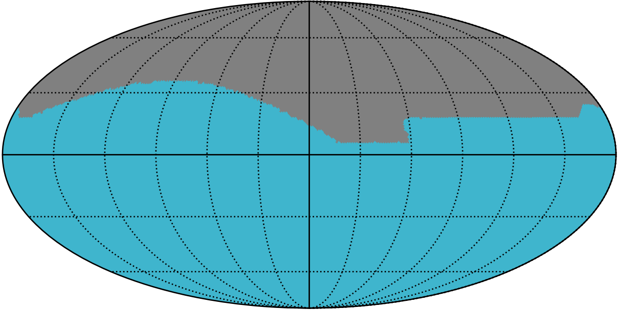
weather_cloudso31v3.4_10yrs : GalplaneFootprintMetric_xray_binaries_map_Tau_2_0
