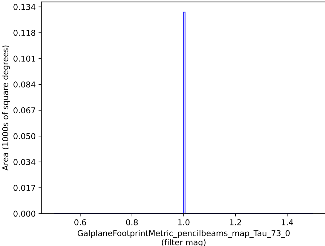
weather_cloudso31v3.4_10yrs : GalplaneFootprintMetric_pencilbeams_map_Tau_73_0
