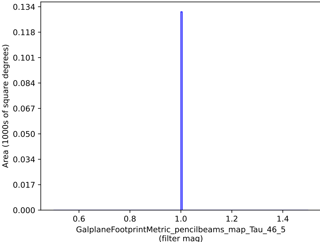
weather_cloudso31v3.4_10yrs : GalplaneFootprintMetric_pencilbeams_map_Tau_46_5
