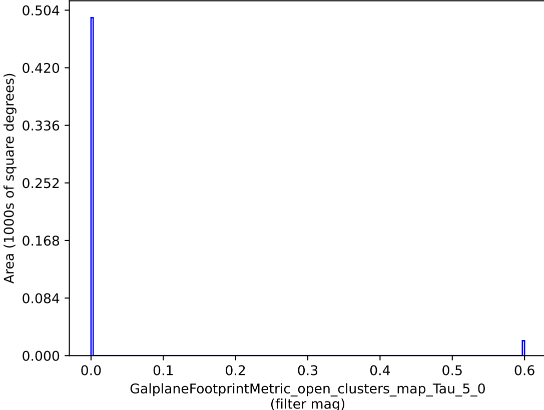
weather_cloudso31v3.4_10yrs : GalplaneFootprintMetric_open_clusters_map_Tau_5_0
