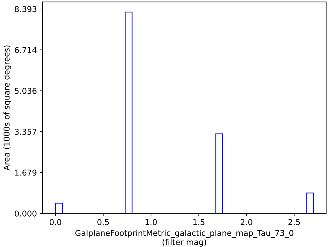
weather_cloudso31v3.4_10yrs : GalplaneFootprintMetric_galactic_plane_map_Tau_73_0
