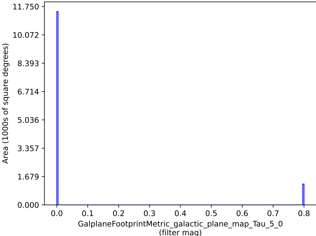
weather_cloudso31v3.4_10yrs : GalplaneFootprintMetric_galactic_plane_map_Tau_5_0
