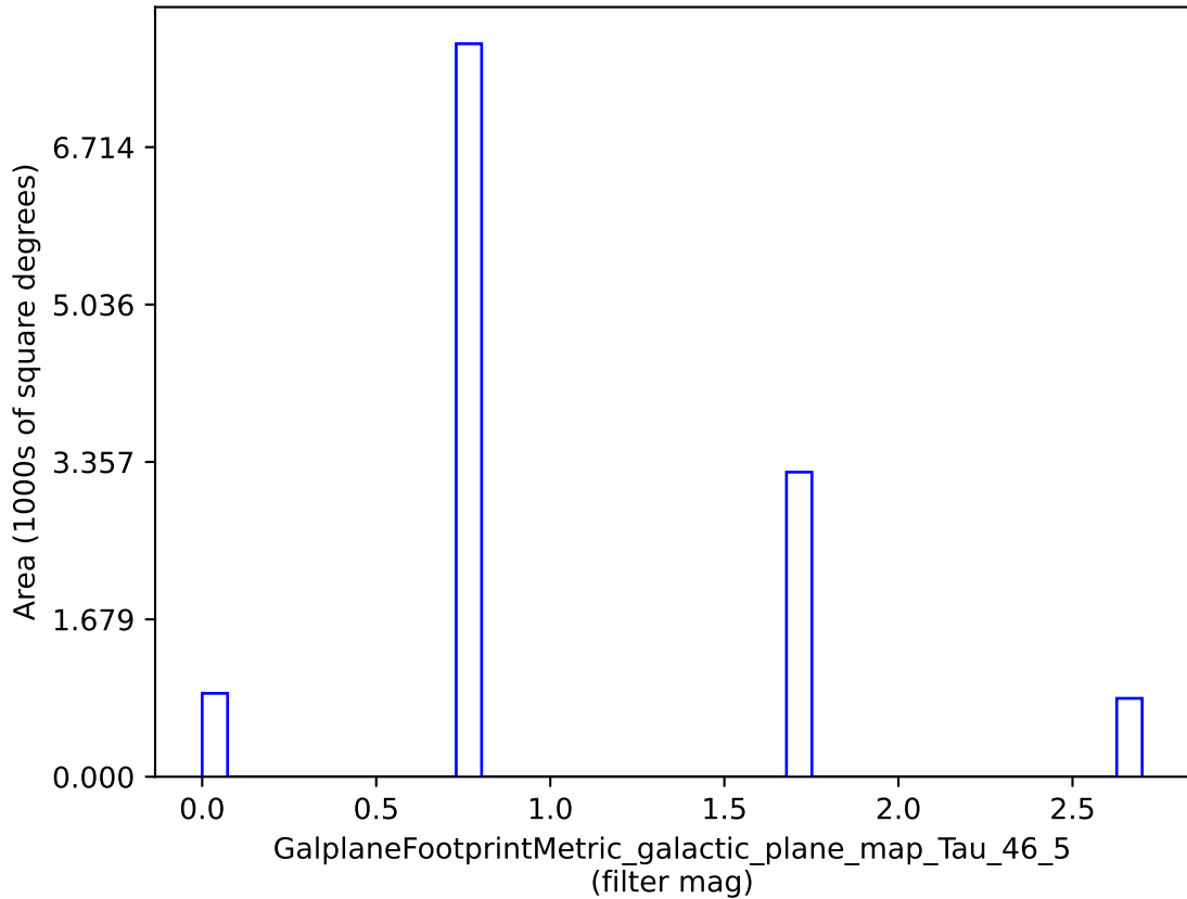
weather_cloudso31v3.4_10yrs : GalplaneFootprintMetric_galactic_plane_map_Tau_46_5
