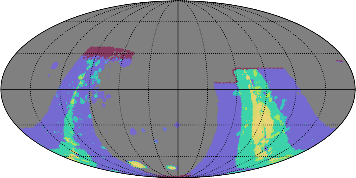
weather_cloudso31v3.4_10yrs : GalplaneFootprintMetric_combined_map_Tau_73_0
