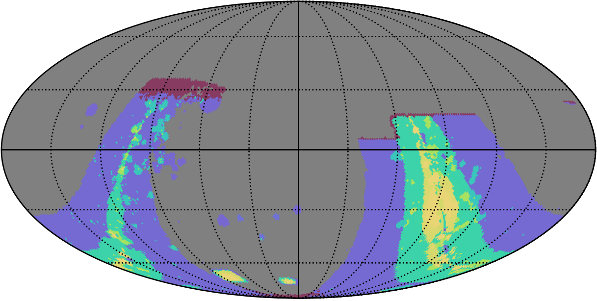
weather_cloudso31v3.4_10yrs : GalplaneFootprintMetric_combined_map_Tau_73_0
