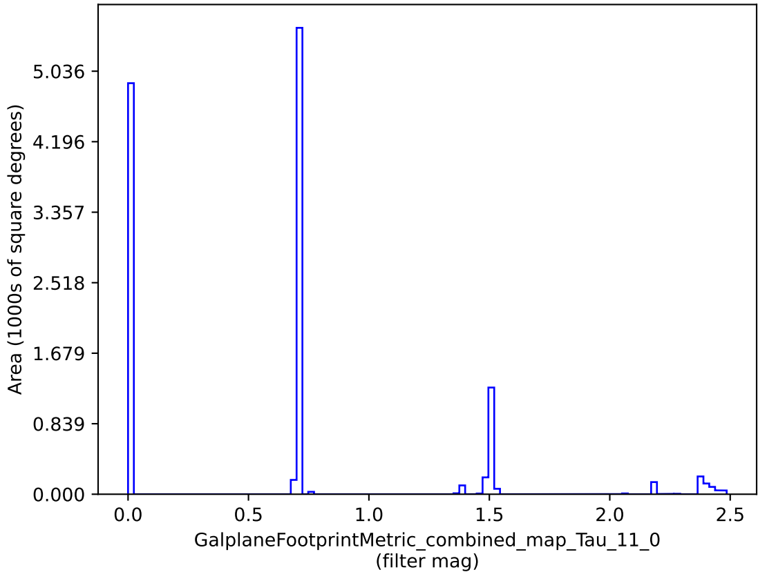
weather_cloudso31v3.4_10yrs : GalplaneFootprintMetric_combined_map_Tau_11_0
