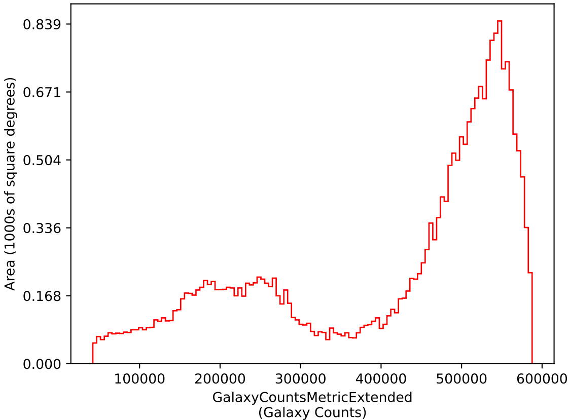
weather_cloudso31v3.4_10yrs i: GalaxyCountsMetricExtended
