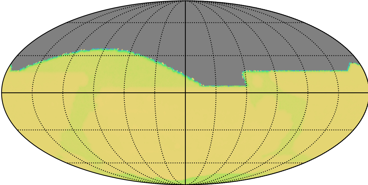
weather_cloudso31v3.4_10yrs : GalPlaneVisitIntervalsTimescales_xray_binaries_map_Tau_73_0
