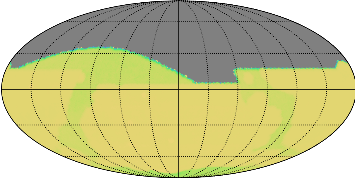
weather_cloudso31v3.4_10yrs : GalPlaneVisitIntervalsTimescales_xray_binaries_map_Tau_46_5
