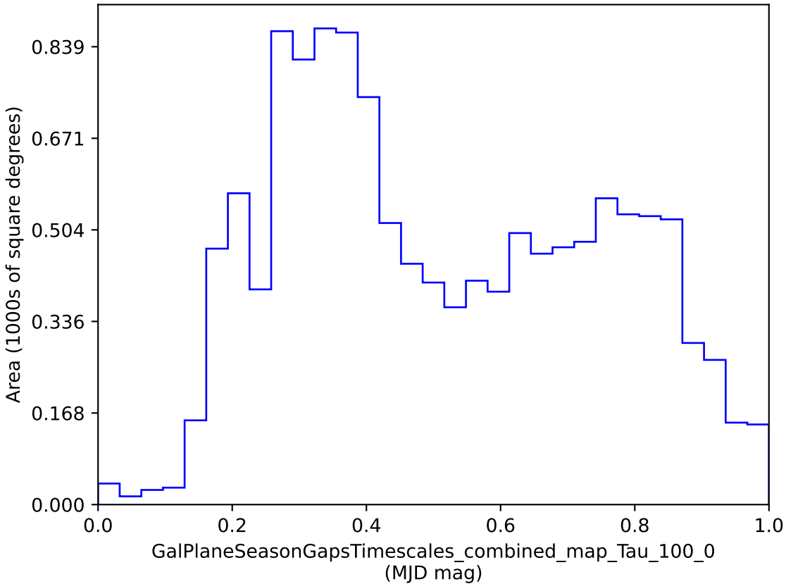
weather_cloudso31v3.4_10yrs : GalPlaneSeasonGapsTimescales_combined_map_Tau_100_0
