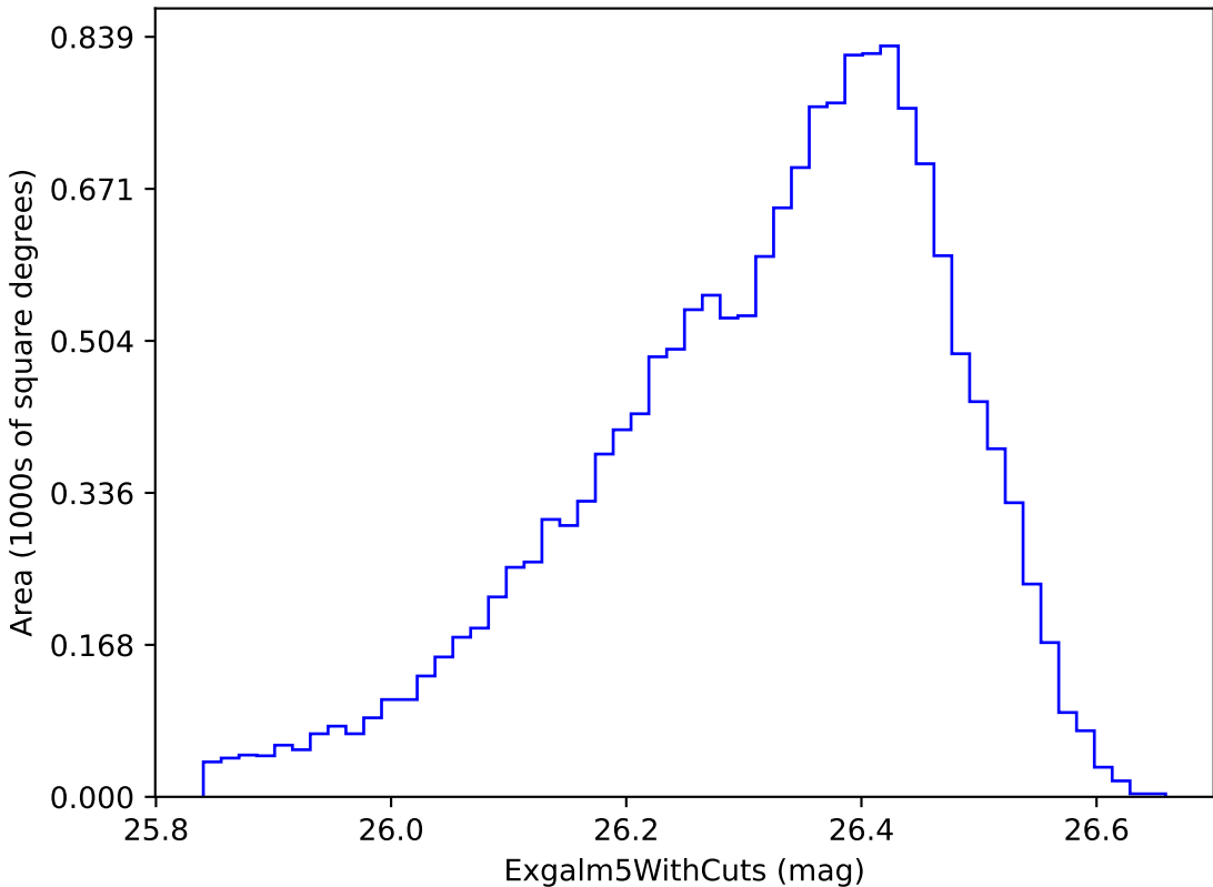
weather_cloudso31v3.4_10yrs i band non-DD year 9: Exgalml5WithCuts
