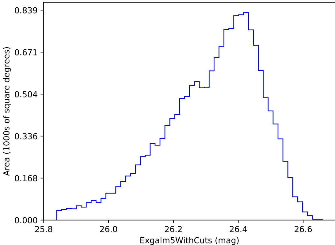
weather_cloudso31v3.4_10yrs i band non-DD year 9: ExgalM5WithCuts
