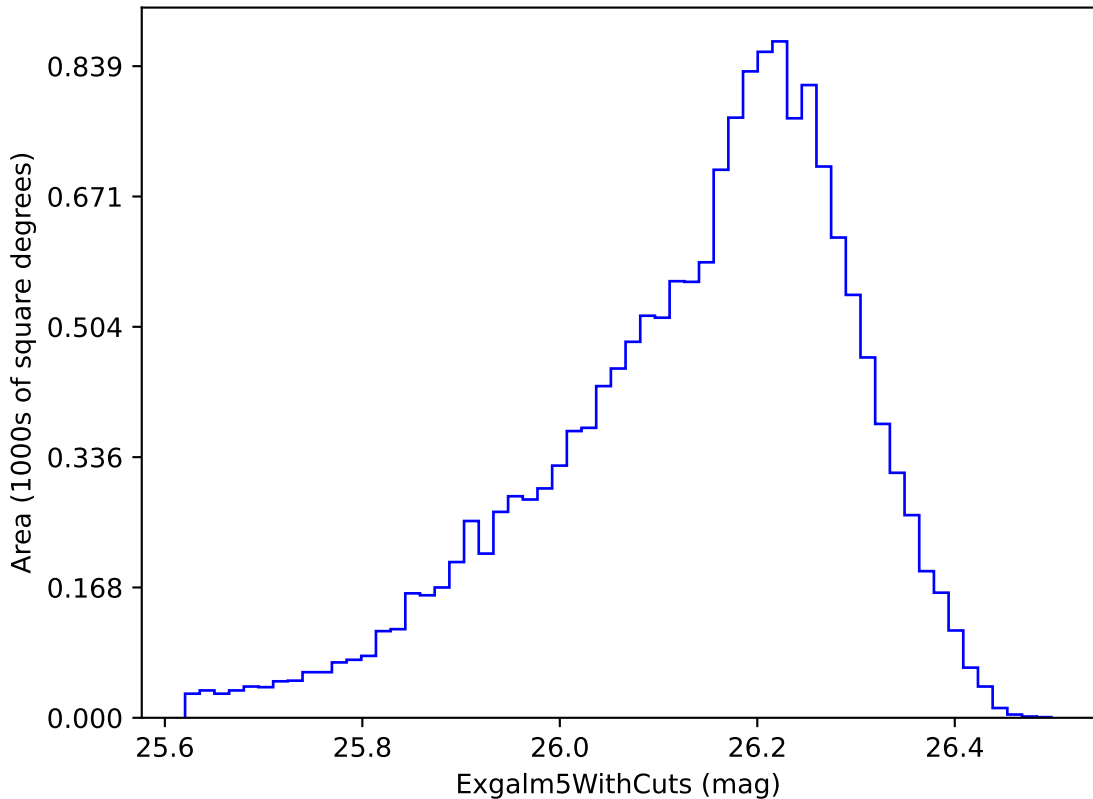
weather_cloudso31v3.4_10yrs i band non-DD year 6: ExgalM5WithCuts
