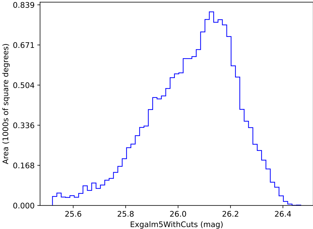
weather_cloudso31v3.4_10yrs i band non-DD year 5: ExgalM5WithCuts
