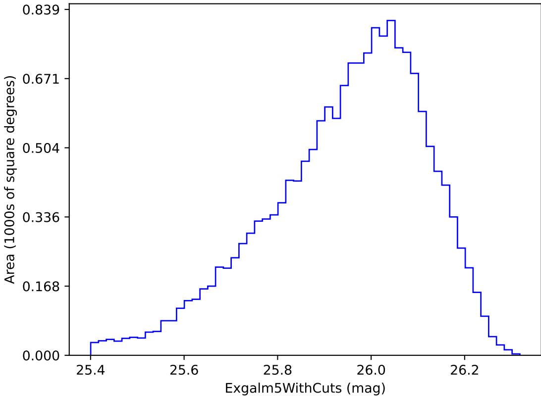
weather_cloudso31v3.4_10yrs i band non-DD year 4: ExgalM5WithCuts
